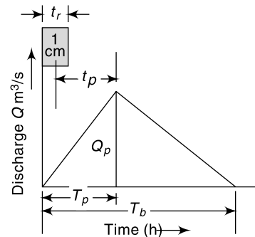
Fig. 6.21(b) SCS Triangular Unit Hydrograph
