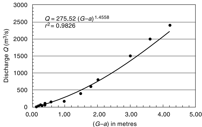
Fig. 4.24(a) Stage-discharge Relation (Arithmetic Plot) – Example 4.4
