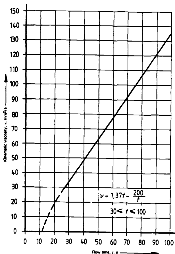
FIG. 3—Calibration curve for 4 mm cup.
