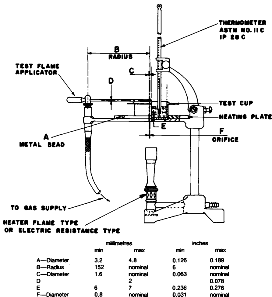
FIG. 1 Cleveland Open Cup Apparatus
