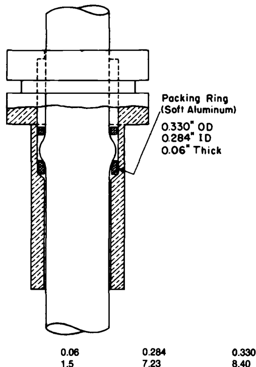
FIG. A3.2 Dimensions for Thermometer Packing Ring (Not Mandatory)
