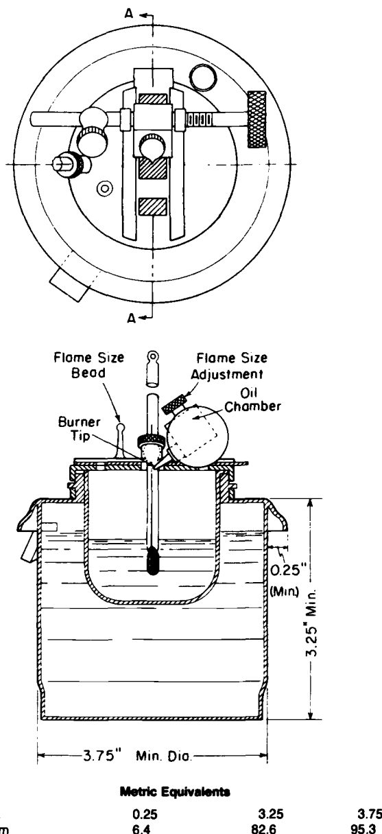
FIG. A1.2 Section of Liquid Bath and Cup
